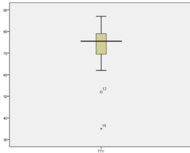
Gambar 2. Data outliers
